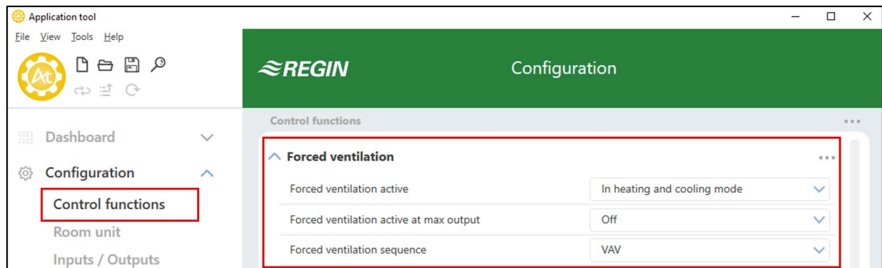
Figure 2-36 Forced ventilation configuration settings in Application tool.
