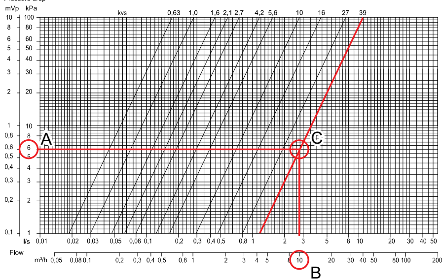
Fig. 3 Example, calculation of the Kv value: At a pressure drop of 6 kPa (A) and a flow of 10 m³ / h (B), the Kv value is 39 (C). See the markings in the picture above.
