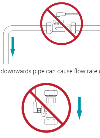
Figure C: downwards curved pipe can collect air-bubble in the proximity of the trasducers.
